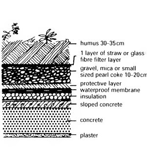
20 Roof garden on a warm roof – protective layer could be replaced by shredded rubber sheet
